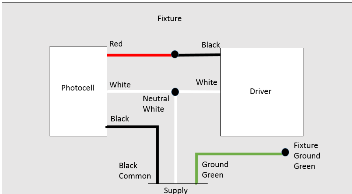
Figure 1: Wiring Schematic
