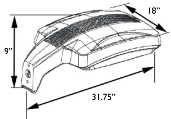
FIGURE 2: DIMENSIONS
